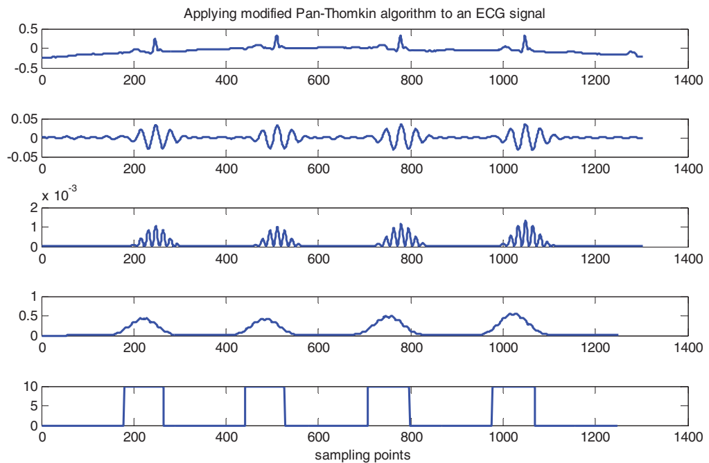
Figure 7.2: Modified Pan-Thompkins algorithm [2] for an ECG signal, from top to bottom: ECG signal, bandpass filtered, squared, moving window integrated and thresholded.
