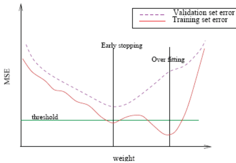
Figure 6.15: Early stopping.
